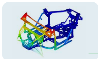
Analysis of the torsional stiffness of a vehicle frame
